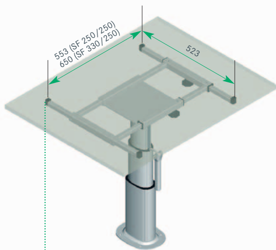
StarLine sliding tabletop fitting 250/250 mm (330/250 mm) – the sliding fitting (SF) can be rotated by 90° as standard.
