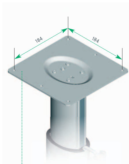
Fixed tabletop connection for the StarLine HPK and HPG
